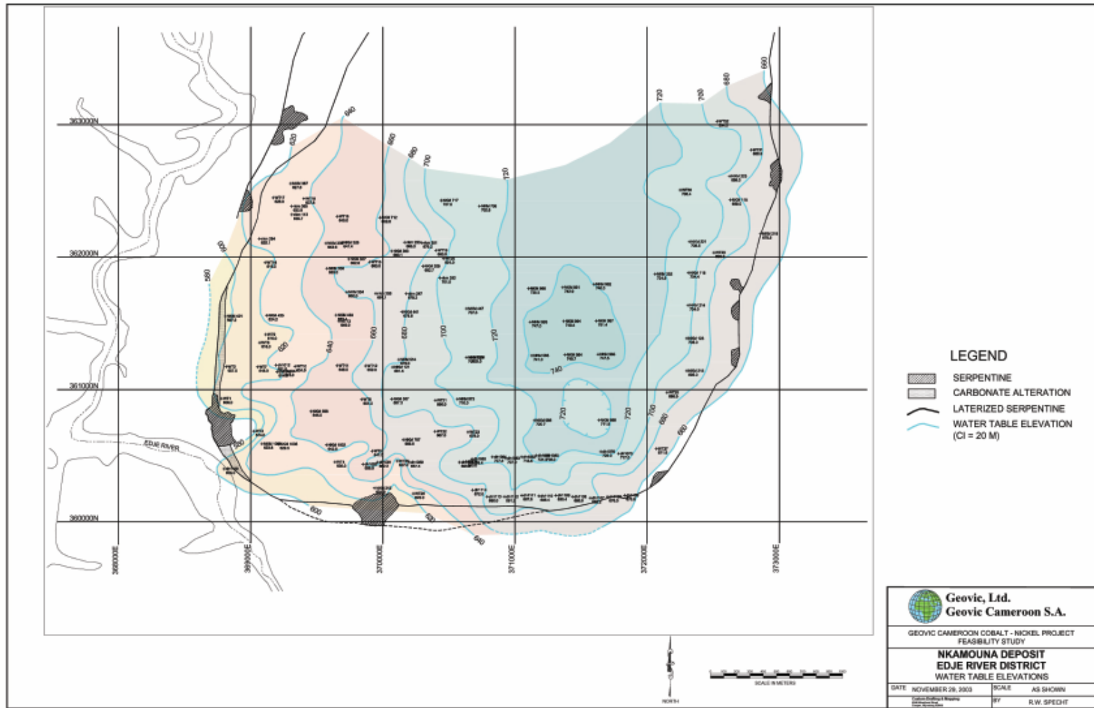
Figure 18. Water Table Elevations
