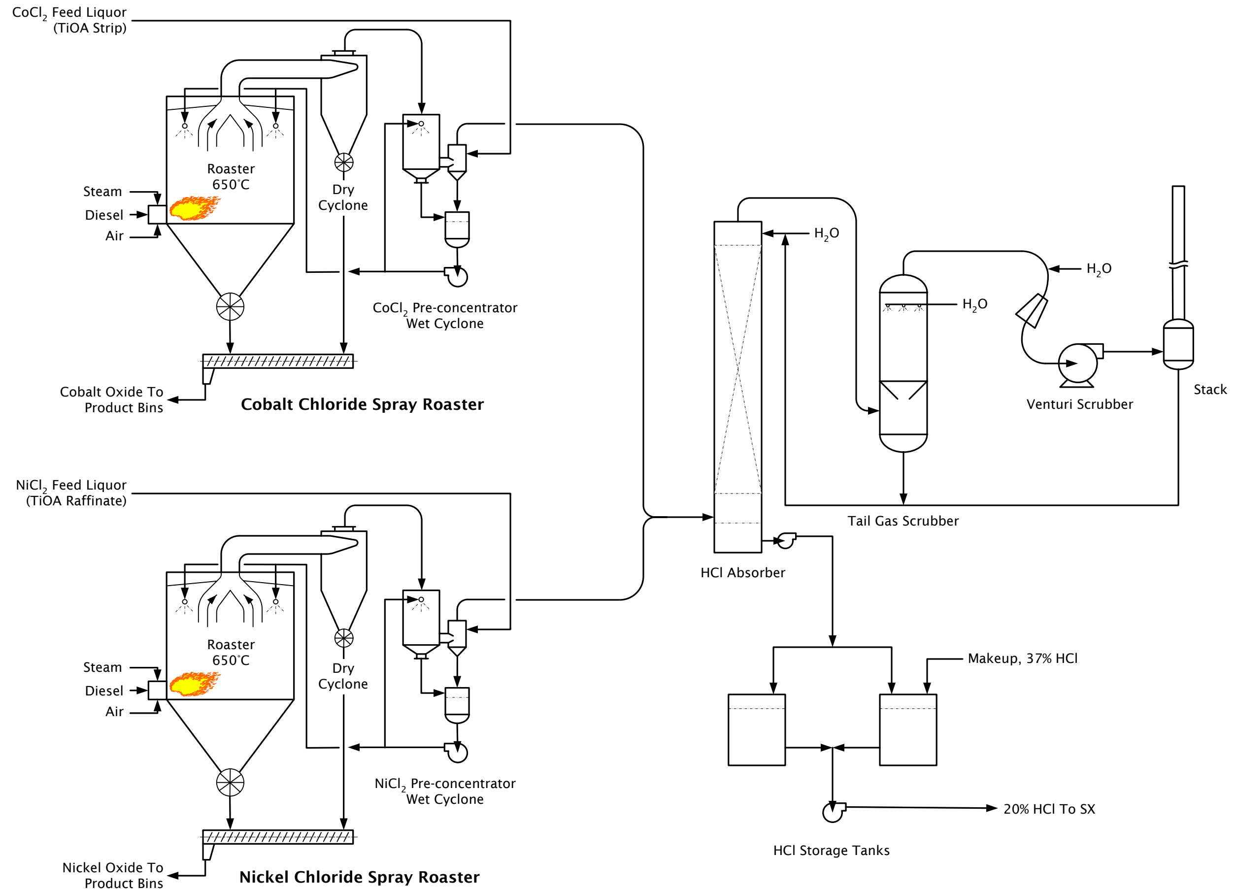
Figure ##. Pyro-hydrolysis, Area 1100
